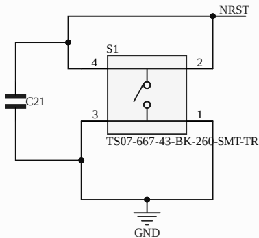
Reset Switch
